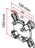
Support universel 100x100 max 20 Nm
